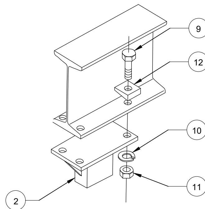
Detail "C"
