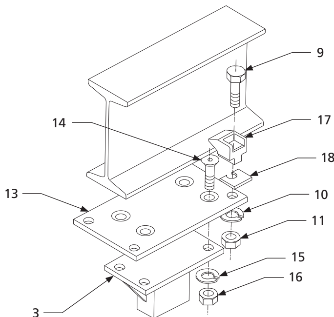
Detail "D"
