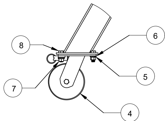
Detail "B" (Caster Assembly)
