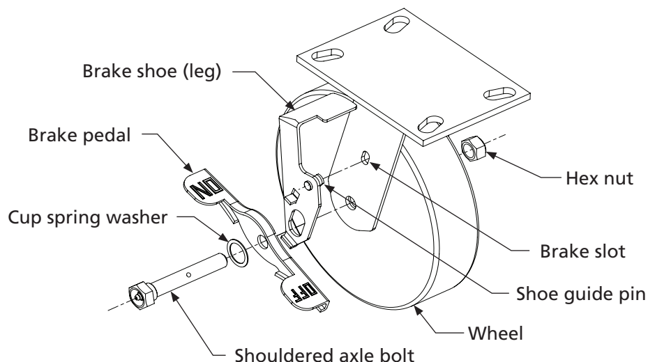
Wheel Brake Assembly Drawing
