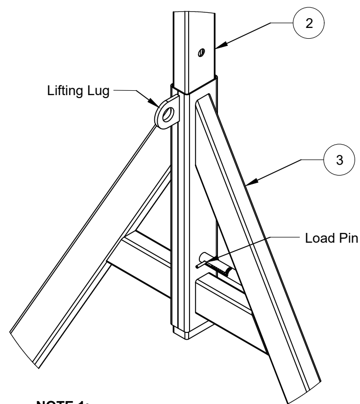
Detail "A"
