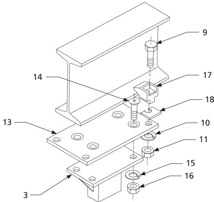
Detail "D"
